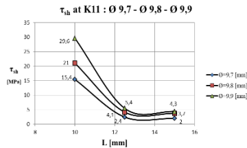
Fig.6 Shear strength of the adhesive-bonded type "shaft-bushing" joint made with K11 adhesive according to the axial length of the contact (L) between the elements at a fixed value of the diameter \varnothing = 9.7; 9.8 and 9.9 mm
