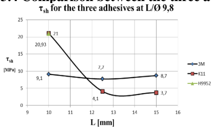
Fig.8 Shear strength of adhesive joint types made with the three types of adhesive depending on the axial length of the contact (L) between the elements at a fixed diameter value \varnothing = 9.8\text{mm}
