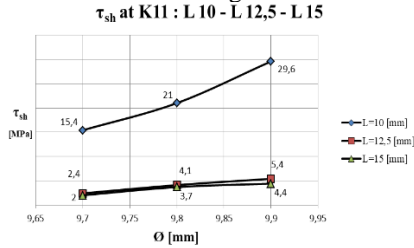
Fig.5 Shear strength of the adhesive-bonded type "shaft-bushing" joint made with K11 adhesive according to the gap between the elements achieved by a different diameter ( \varnothing ) of the pin.
