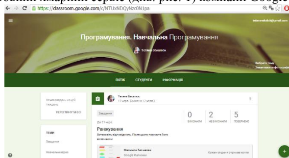
Рис. 1. Google Classroom
